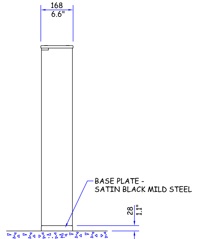
END VIEW
